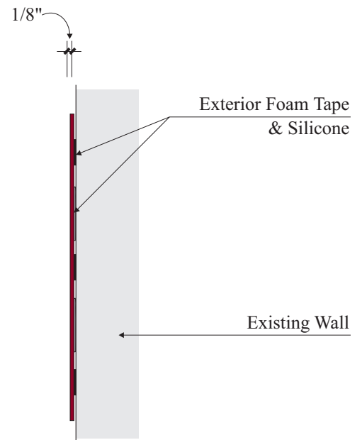
Side Views
